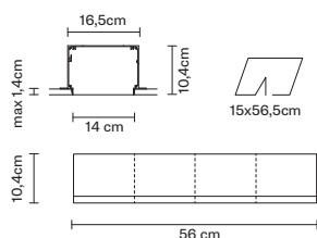
CASSAFORMA 14x56 cm / WALLBOX 14x56 cm
