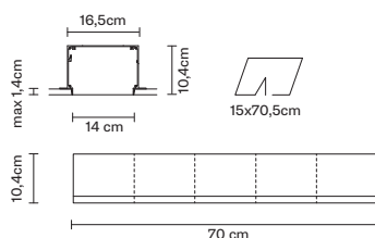
CASSAFORMA 14x70 cm / WALLBOX 14x70 cm
